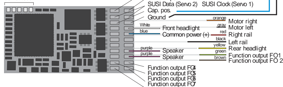
MX645 wires only Top Side
